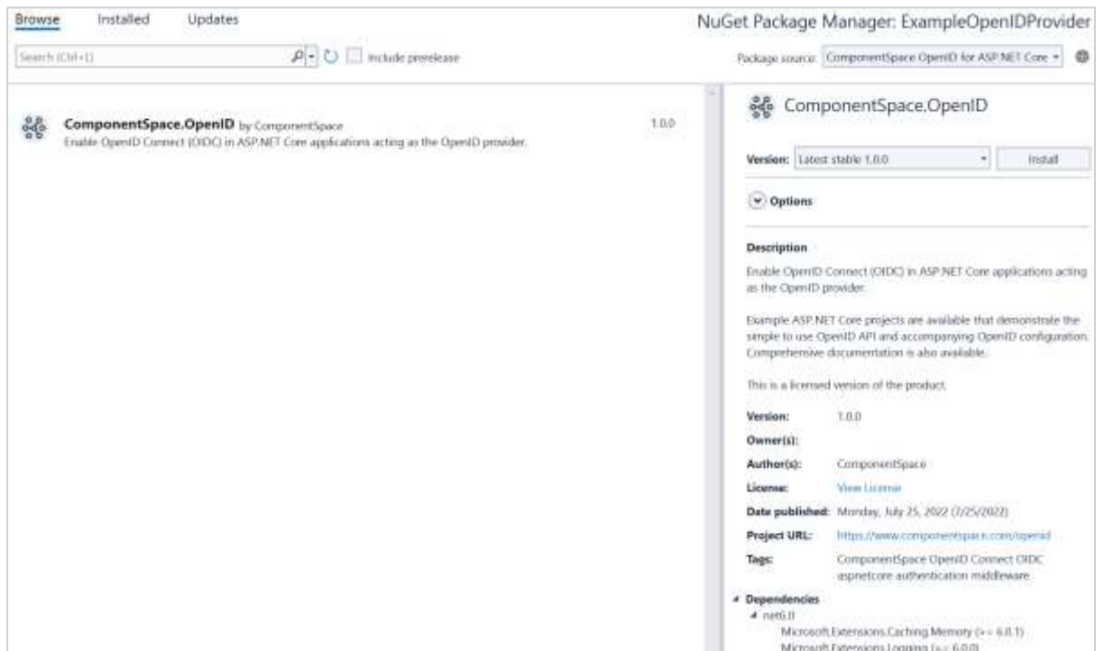
Figure 4 Install ComponentSpace.OpenID
